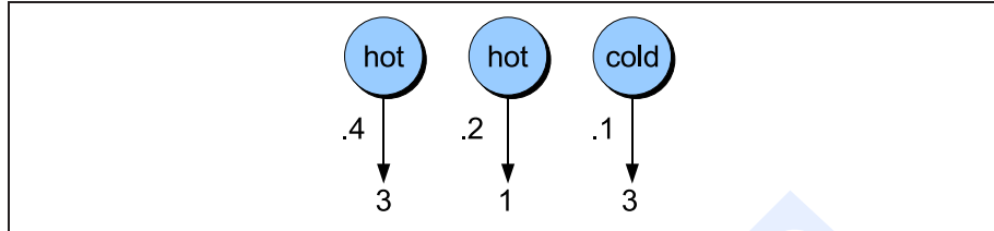
Figure 6.5 The computation of the observation likelihood for the ice-cream events 3 1 3 given the hidden state sequence hot hot cold.
