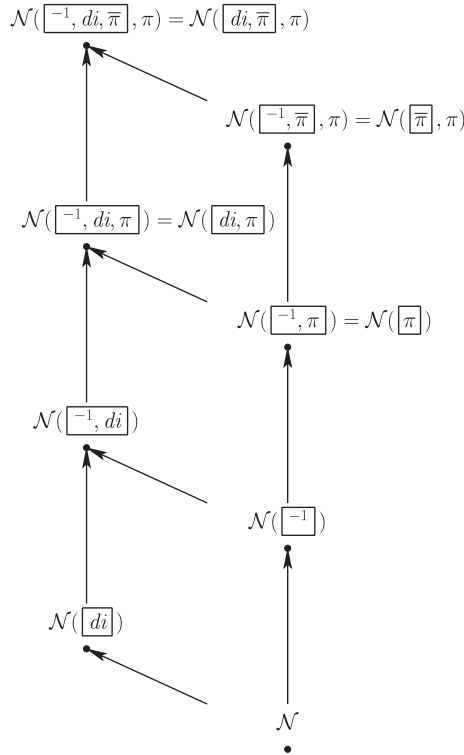
Fig. 7. The Hasse diagram of \leq^{\text{bool}} for \mathcal{C} . For each language, the boxed features are a minimal set of nonbasic features defining the language, while the other features can be derived from them in the sense of Theorem 5.2 (using the appropriate interdependencies).
