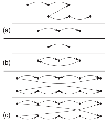
Fig. 4. Graph pairs used to prove \not\leq_{\text{strong}}^{\text{bool}} results in Sections 5 and 6. All edges are assumed to have the same label R .
