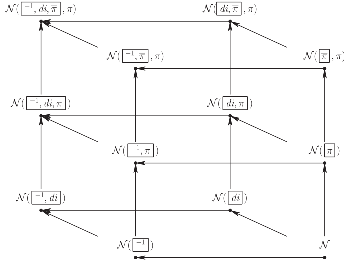
Fig. 3. The Hasse diagram of \leq^{\text{path}} for \mathcal{C} . For each language, the boxed features are a minimal set of nonbasic features defining the language, while the other features can be derived from them in the sense of Theorem 5.2 (using the appropriate interdependencies).
