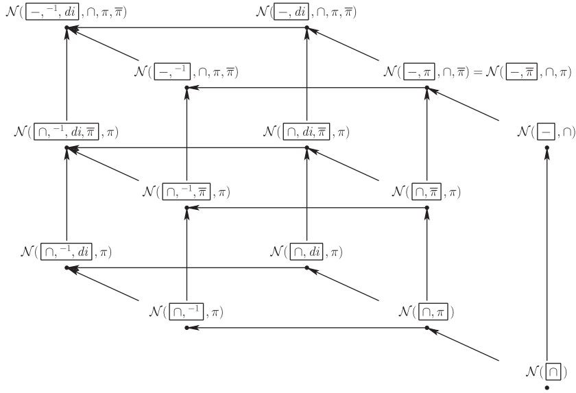
Fig. 6. The Hasse diagram of \leq^{\text{path}} and \leq^{\text{bool}} for \mathcal{C}[\cap] .
