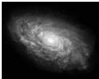
(a) A spiral galaxy.
